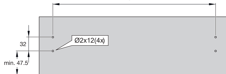
Cote prelucrare front LW-31
